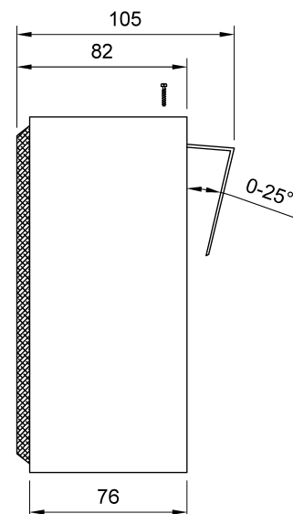
RIGHT VIEW
