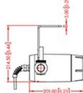
SIDE VIEW Ceiling mount
