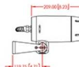
SIDE VIEW Wall Mount
